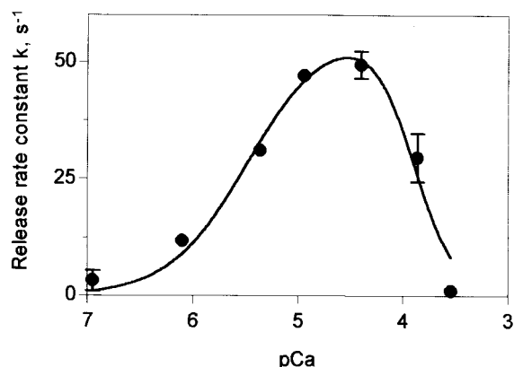
FIGURE 1 Effect of increasing extravesicular [\text{Ca}^{2+}] on the rate constants of calcium release. Triads were passively equilibrated with 2 mM \text{CaCl}_2 and were diluted 1:10 with solutions that, after mixing, had the variable free [\text{Ca}^{2+}] indicated in the figure plus 1.20 \pm 0.02 mM free [ATP] (mean \pm SD). The rate constants of calcium release were obtained from single exponential fitting of experimental records such as those shown in Fig. 2. To cover the pCa range indicated in the figure, different calcium indicators were used. Fluo-3 ( K_D = 0.39 \mu\text{M} ) was used in the pCa range 7.0–6.0; Calcium Green-2 ( K_D = 0.59 \mu\text{M} ) for the pCa range 6.0–4.9; Calcium Green-5N ( K_D = 27.5 \mu\text{M} ) for the pCa range 4.9–3.9, and Fluo-5N ( K_D = 90 \mu\text{M} ) for pCa values ranging from 3.9 to 3.5. For further details, see text.
