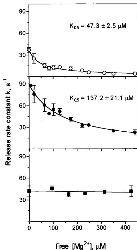
FIGURE 3 Effect of [\text{Mg}^{2+}] on calcium release rate constants in native and oxidized triads passively loaded with calcium. The rate constants k of calcium release were calculated from single exponential fitting of experiments such as those shown in Fig. 2. The solid line represents the best fitting to the equation: k = k_{\text{max}} K_{0.5} / ([\text{Mg}^{2+}] + K_{0.5}) , where k_{\text{max}} is the value of k in the absence of \text{Mg}^{2+} and K_{0.5} represents the concentration of \text{Mg}^{2+} that produced 0.5 k_{\text{max}} . Open symbols: native triads; filled circles: triads oxidized with 500 \mu\text{M} thimerosal for 5 min; filled squares: triads oxidized with 500 \mu\text{M} thimerosal for 10 min. Data are given as mean \pm SEM.
