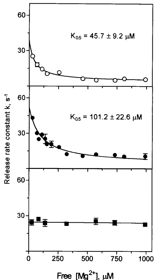
FIGURE 4 Effect of [\text{Mg}^{2+}] on calcium release rate constants in native and oxidized triads that were endogenously phosphorylated during active calcium loading. The rate constants k of calcium release were calculated from single exponential fitting of experiments such as those shown in Fig. 2. The solid line represents the best fitting to the equation: k = k_{\text{max}} K_{0.5} / ([\text{Mg}^{2+}] + K_{0.5}) , where k_{\text{max}} is the value of k in the absence of \text{Mg}^{2+} and K_{0.5} represents the concentration of \text{Mg}^{2+} that produced 0.5 k_{\text{max}} . Open symbols: native triads; filled circles: triads oxidized with 250 \mu\text{M} thimerosal for 1 min; filled squares: triads oxidized with 500 \mu\text{M} thimerosal for 10 min. Data are given as mean \pm SEM.
