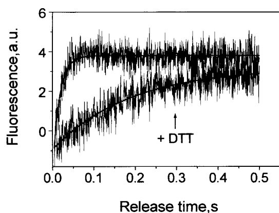
FIGURE 6 Reversibility of the oxidation of triads with thimerosal. Triads passively loaded with calcium were oxidized with 500 \mu\text{M} thimerosal for 5 min and were further incubated with 5 mM DTT for 5 min before inducing CICR as in Fig. 2. The free [\text{Mg}^{2+}] of the releasing solution was 129 \mu\text{M} . Each trace was obtained by averaging three different traces. The solid line represents the fitting to a single exponential function.
